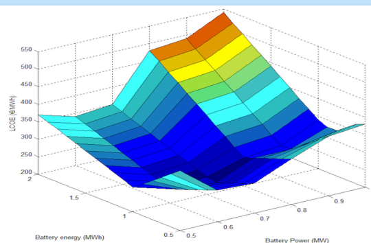
Results of the simulation with LCOE as an optimization metric
