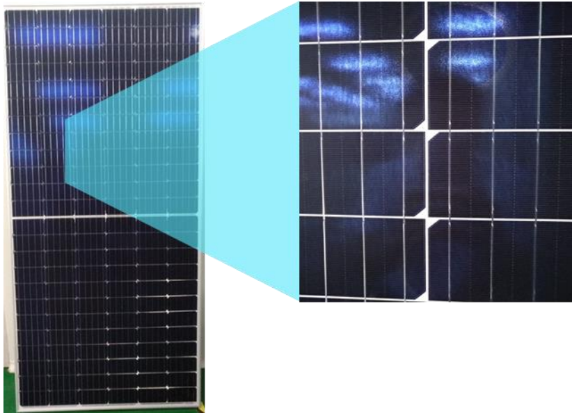
Fig. 4. 385W half PERC cell (144) + LRF over the ribbons module. Enlargement to show precise LRF alignment over ribbons.
